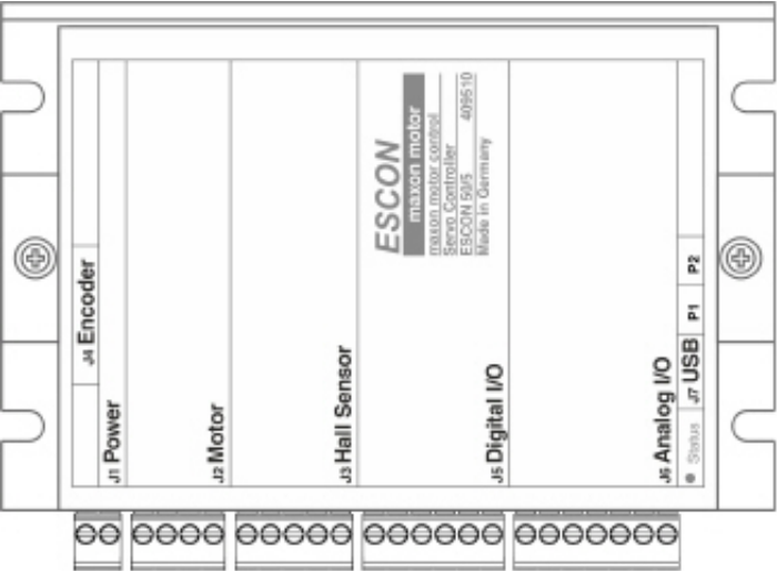
Figure 1-3 Interfaces – Location
