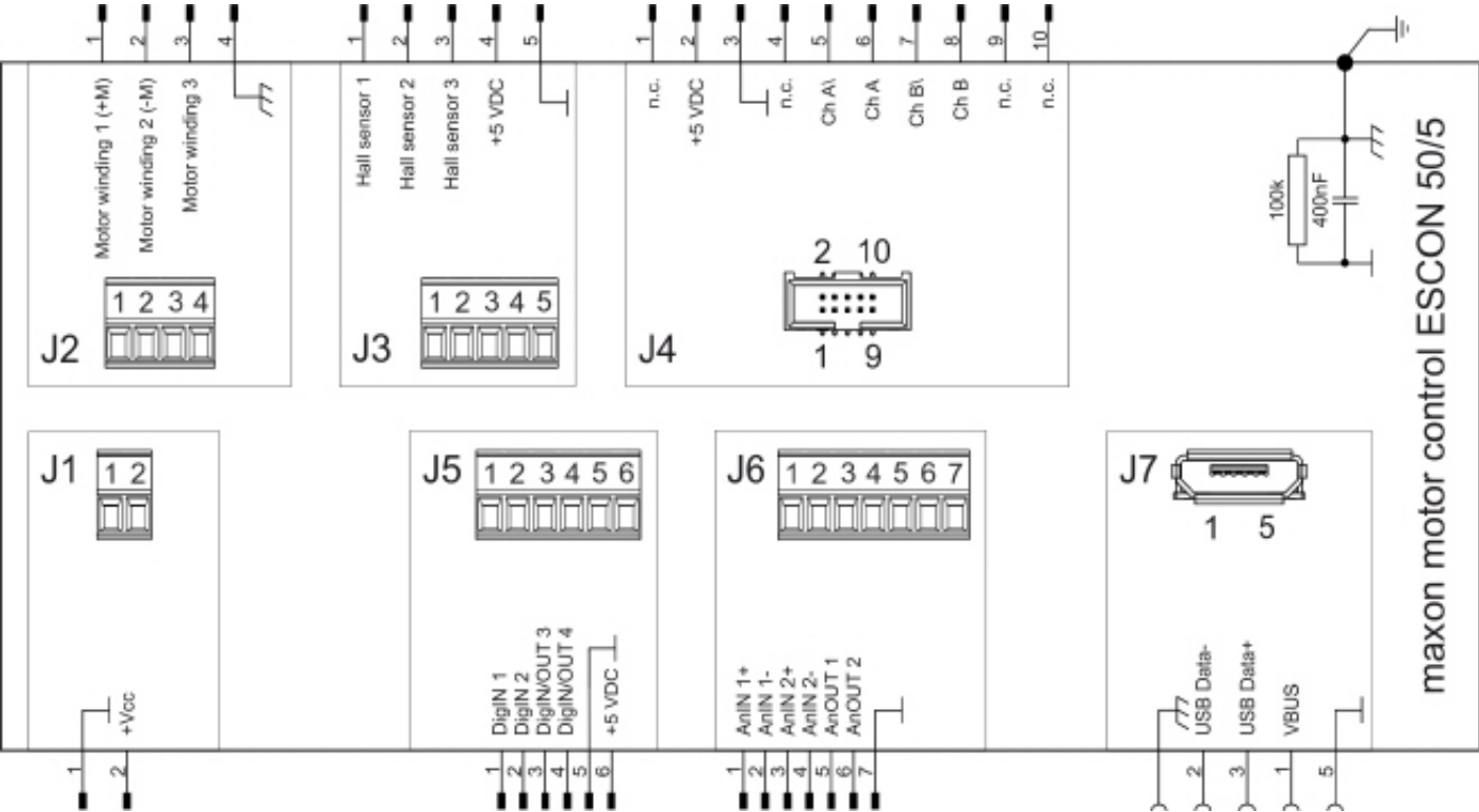
Figure 1-4 Interfaces – Pin Assignment
